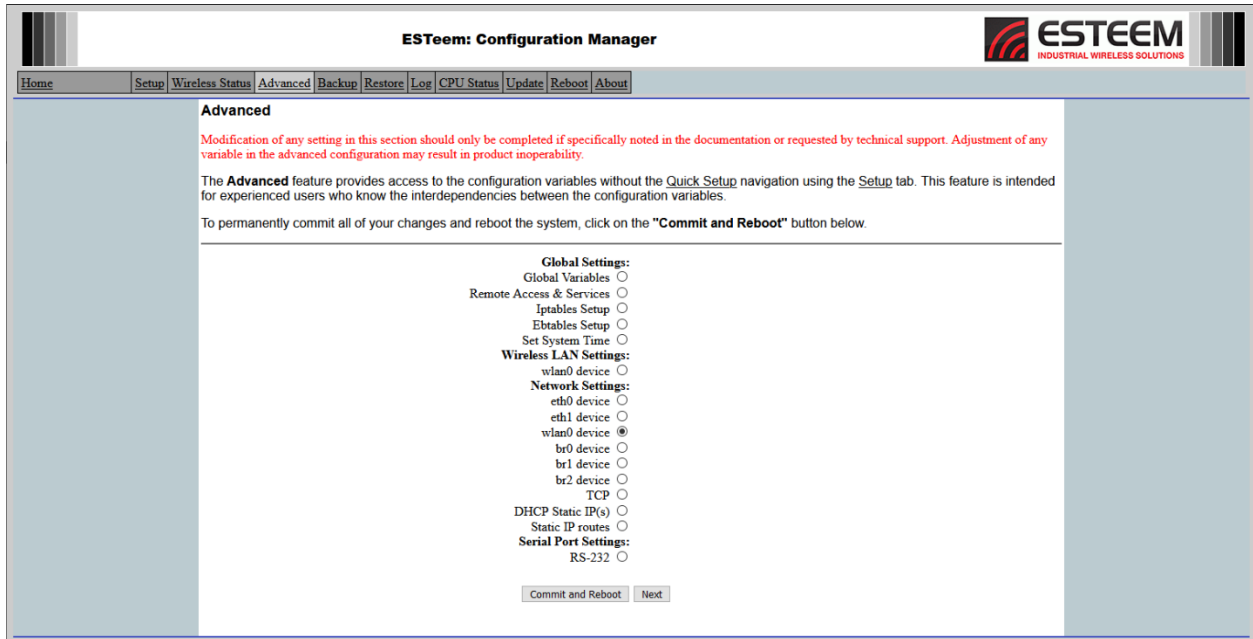
Figure 3: Advanced Settings
