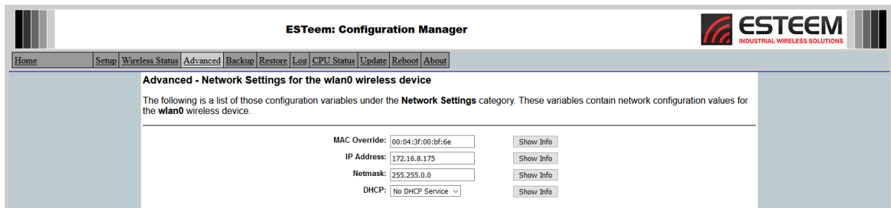
Figure 4: wlan0 Settings
