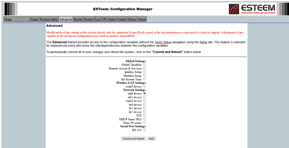
Figure 1: Advanced Screen
