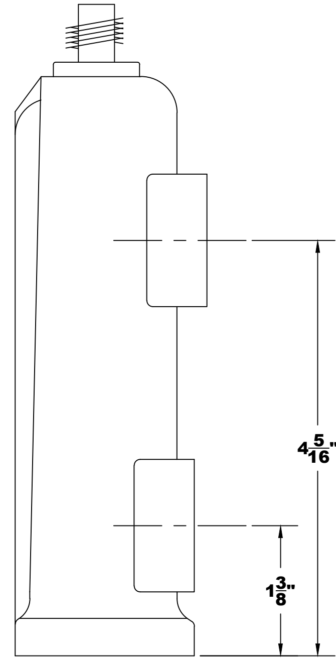
SIDE VIEW
