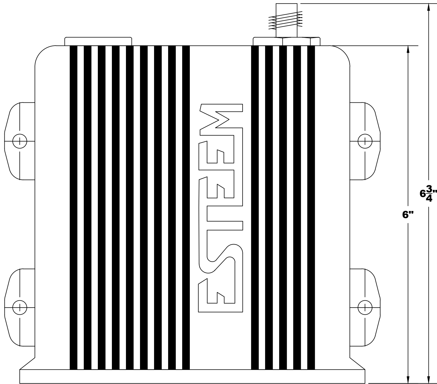
TOP VIEW
